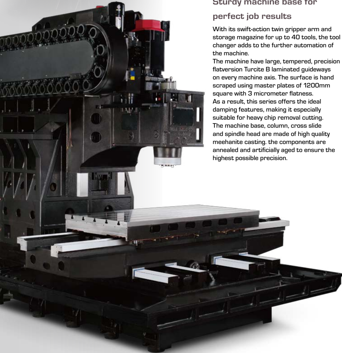
Fig.: Machine base AA1680
